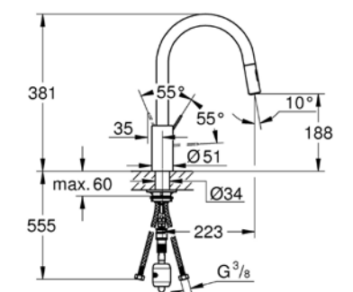
Eurosmart Cosmopolitan 31481001 (1000534) 伸縮廚房龍頭
